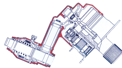
A320 Flap Operating System Rotary Actuator & Offset Gearbox
